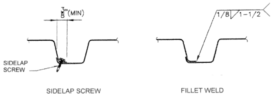
FIGURE 3—SIDELAP FASTENER DETAILS
