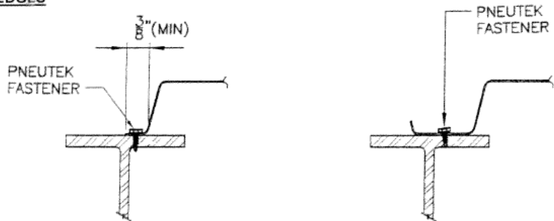
FIGURE 2—PNEUTEK FRAME (SUPPORT) FASTENER DETAILS
