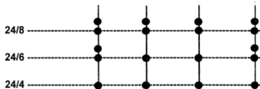
FIGURE 1—PNEUTEK SUPPORT FASTENER PATTERNS AND DECK PROFILES
